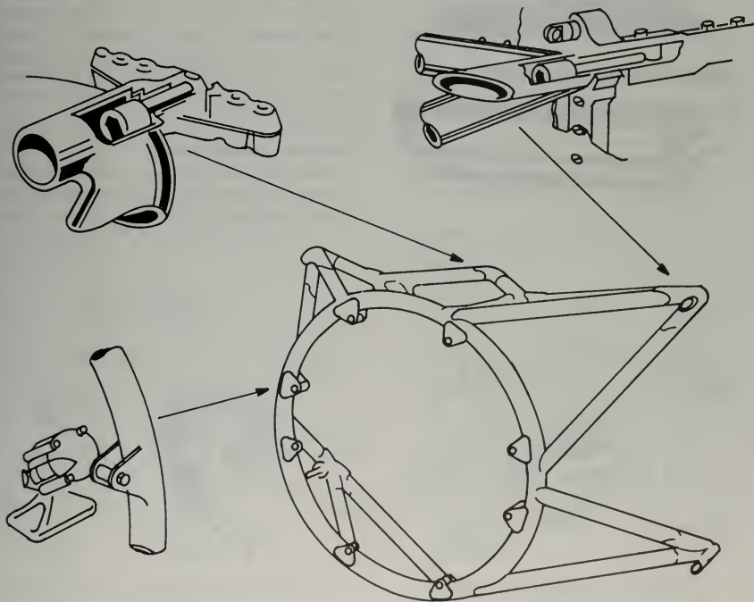
FIGURE 8-25. Typical engine mount.
